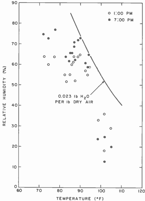
Fig. 2—The average daily maximum temperatures for the 3 hottest months versus the average relative humidity for each of these months at 1:00 PM (open circles) and 7:00 PM (filled circles) for six cities in the U.S. (Atlanta, Baltimore, Houston, Miami, Phoenix, and San Diego). The solid curve shows the relative humidity versus temperature for an absolute humidity of 0.023 pound of water per pound of dry air. This curve served as a basis for establishing certain coatings stress tests. For example, 85°F and 90% RH is used for accelerating the corrosive effects and adhesion of applications of controlled quantities of house dust.
