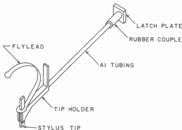
Fig. 12—Stylus support arm.
