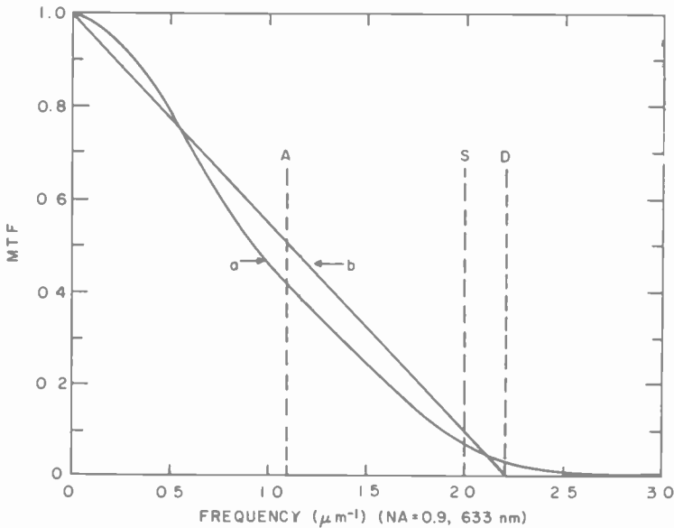
Fig. 8—Modulation transfer function of a commercially available, high quality microscope objective (NA = 0.9). A is the axial-detector cutoff frequency, S the spatial frequency corresponding to the shortest VideoDisc signal wavelength, and D is the split-detector cutoff frequency.
