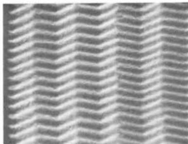
(b) VIDEO PROGRAM PATTERN ON 9541 GROOVES/in. DISC AT INSIDE RADIUS 10k × MAG.
