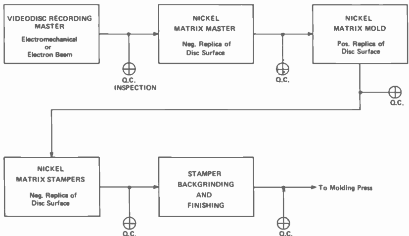
Fig. 10—VideoDisc matrix process flow sequence.
