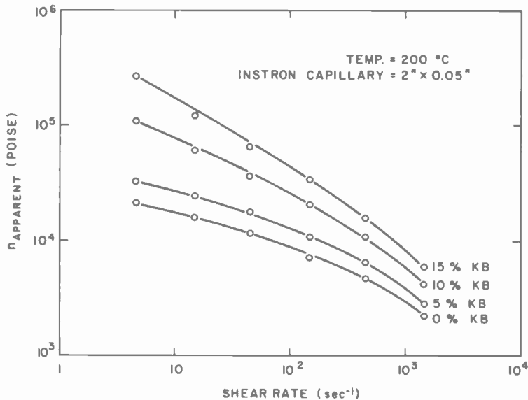
Fig. 9—The effect of carbon loading on the apparent viscosity of a propylene-vinyl chloride copolymer.
