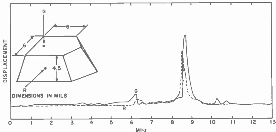
Fig. 15—Experimental cutter head transducer movement measured interferometrically. The peak of trace G corresponds to approximately 0.002 \mu\text{m} peak-to-peak transducer displacement.
