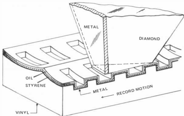
Fig. 1 —Cutaway view of stylus tip and coated VideoDisc surface. This figure represents an early stage of development. The stylus shape and the form of the information recorded in the grooves are different in the current system.
