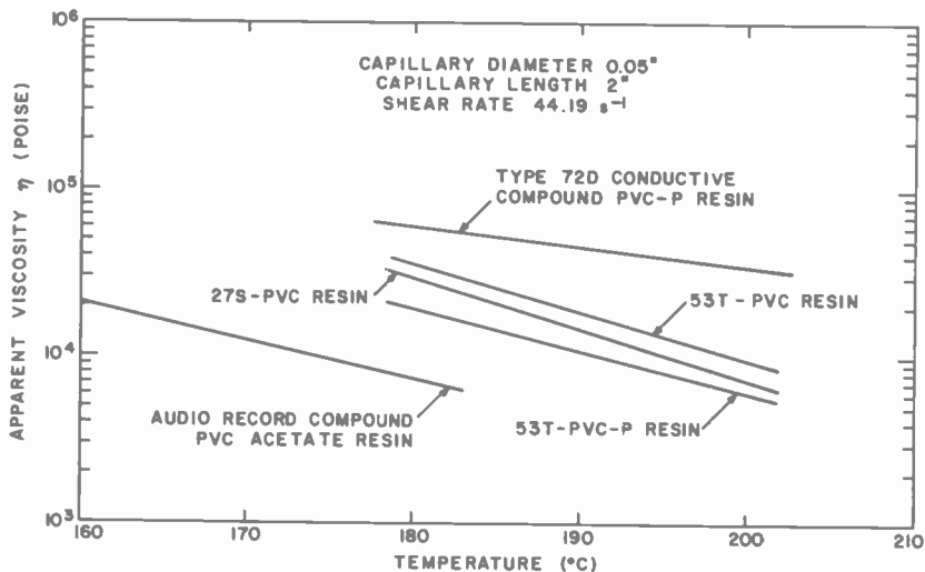
Fig. 4—Melt viscosity versus temperature characteristics of various compounds.
