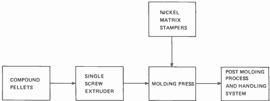
Fig. 9—VideoDisc molding process flow sequence.
