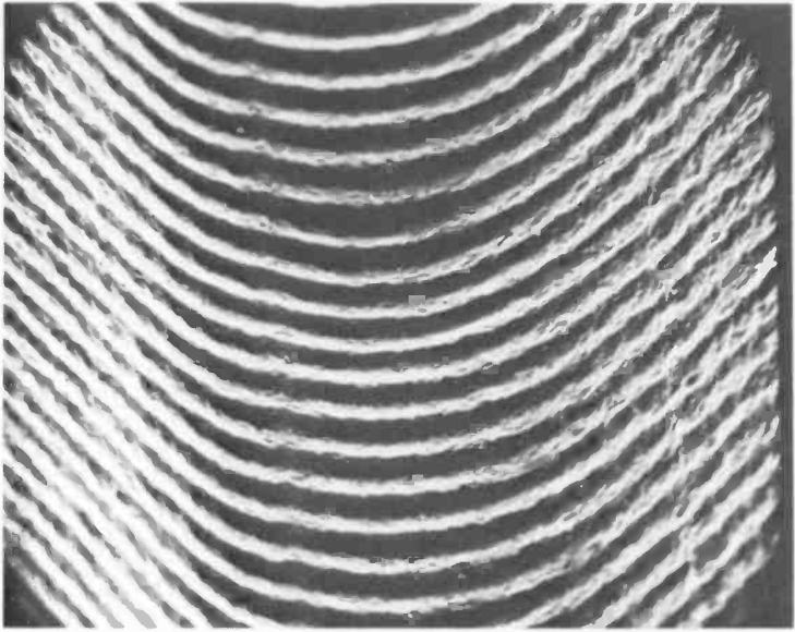
Fig. 18 —Surface quality of signal mechanically cut in lacquer. The width of the signal groove shown here is 12\ \mu\text{m} .
