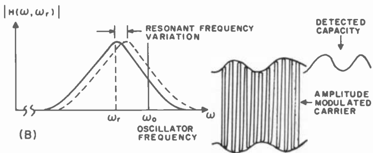
Fig. 3—Capacitance detection: (A) detection circuitry and (B) circuit signal responses.
