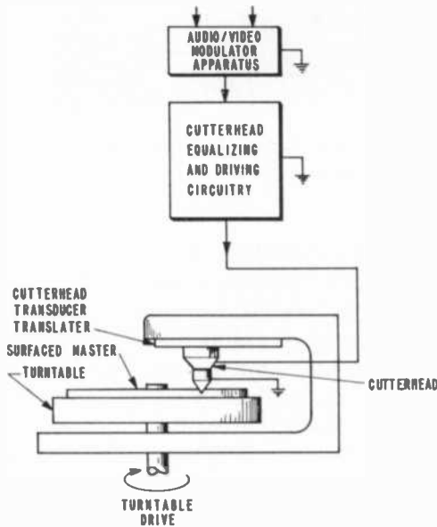
Fig. 17—Simplified schematic diagram of an electromechanical recorder.
