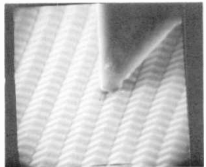
Fig. 1—Left: Schematic drawing of the capacitive stylus in a groove on a VideoDisc. Right: Scanning electron micrograph showing the trailing (electrode) edge of a diamond stylus on a 9524 groove-per-inch electromechanically-mastered (V-groove) disc.
