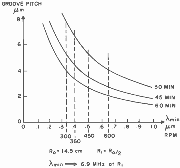
Fig. 11—Groove pitch versus \lambda_{\text{min}} for various playing times and RPM with R_i = R_0/2 .
