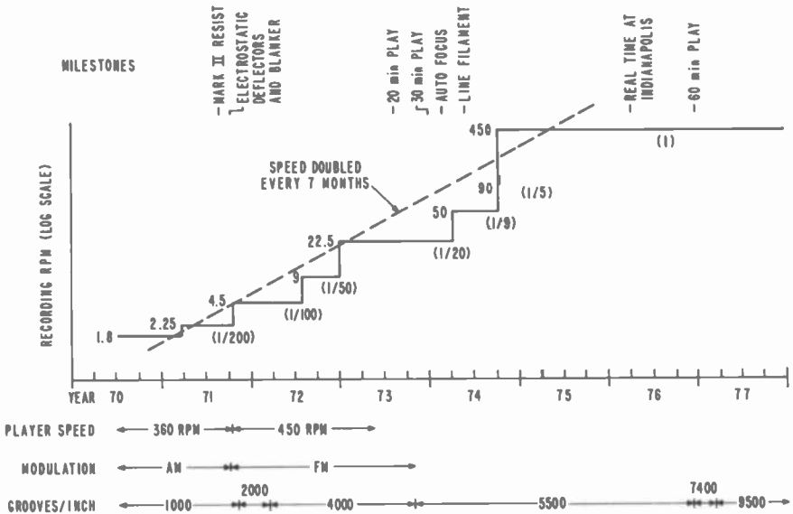
Fig. 3—Chart showing the chronological improvement in electron-beam mastering speed along with mastering and system steps related to the speed increases.
