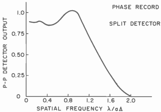
Fig. 6—Square-wave frequency response of a differential-phase split detector. Peak-to-peak detector output, normalized to unity at the frequency of maximum output, is plotted as a function of spatial frequency for an optimum-depth, \pi/2 -phase-shift, square-wave phase grating.
