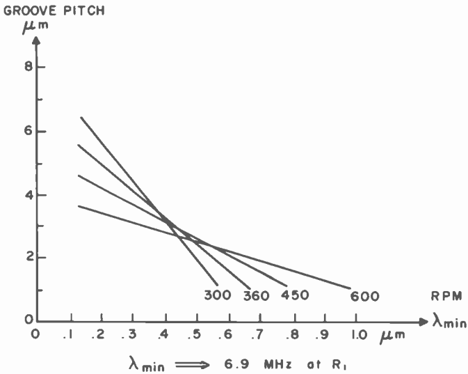
Fig. 12—Groove pitch versus \lambda_{\text{min}} for various RPM for a 60-minute disc.
