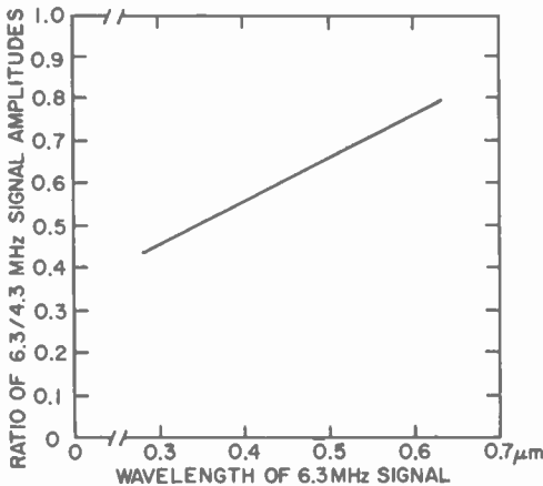
Fig. 13—Signal amplitude versus spatial wavelength.
