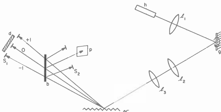
Fig. 11—Schematic outline of the optical system of a VideoDisc defect detector.
