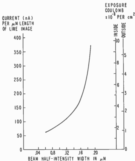
Fig. 8—Beam current per \mu\text{m} length of a line image versus line width at half-intensity level.
