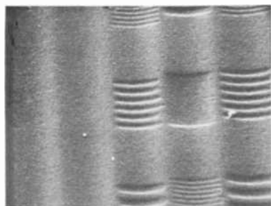
(a) TEST SIGNALS AT 4.2, 6.3, AND 12.6 MHz ON 5555 GROOVES/in. DISC AT INSIDE RADIUS 5k × MAG.
