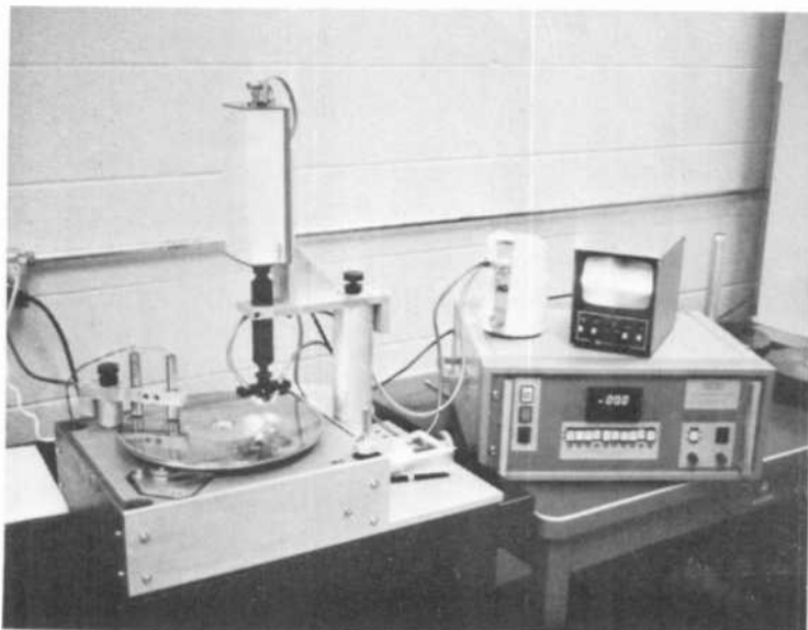
Fig. 5—Warp/TIR test station.
